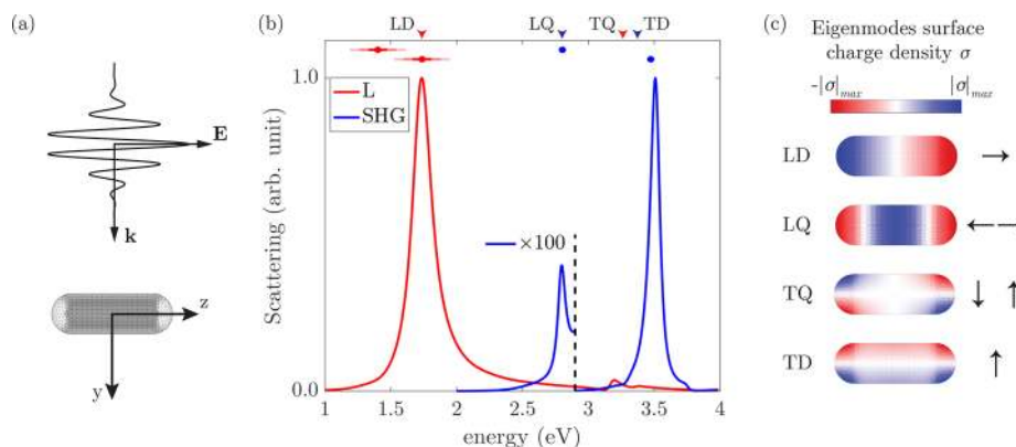
Figure 2. (a) Sketch of the excitation configuration. (b) Plane-wave scattering spectrum, linear monochromatic response (red curve), and corresponding SHG (blue curve). The SHG on the left of the vertical dashed line is multiplied by a factor 100 to highlight the resonance of the LQ mode. The red dots and horizontal lines respectively indicate the central energies \omega_0 and width 2\Delta\omega_0 at the fundamental stage for the pulses used here. The blue dots give the central frequency of the corresponding nonlinear excitation P_{\text{NL}} without taking into account the influence of the linear response, i.e., \omega_0^{\text{NL}} = 2\omega_0 . The position of the eigenmodes presented in (c) are shown on the top abscissa. (c) Surface charge distributions \sigma of the four eigenmodes discussed here. LD stands for longitudinal dipole, LQ for longitudinal quadrupole, TD for transverse dipole, and TQ for transverse quadrupole; see Table 1. Black arrows represent the local dipolar moment orientations.
