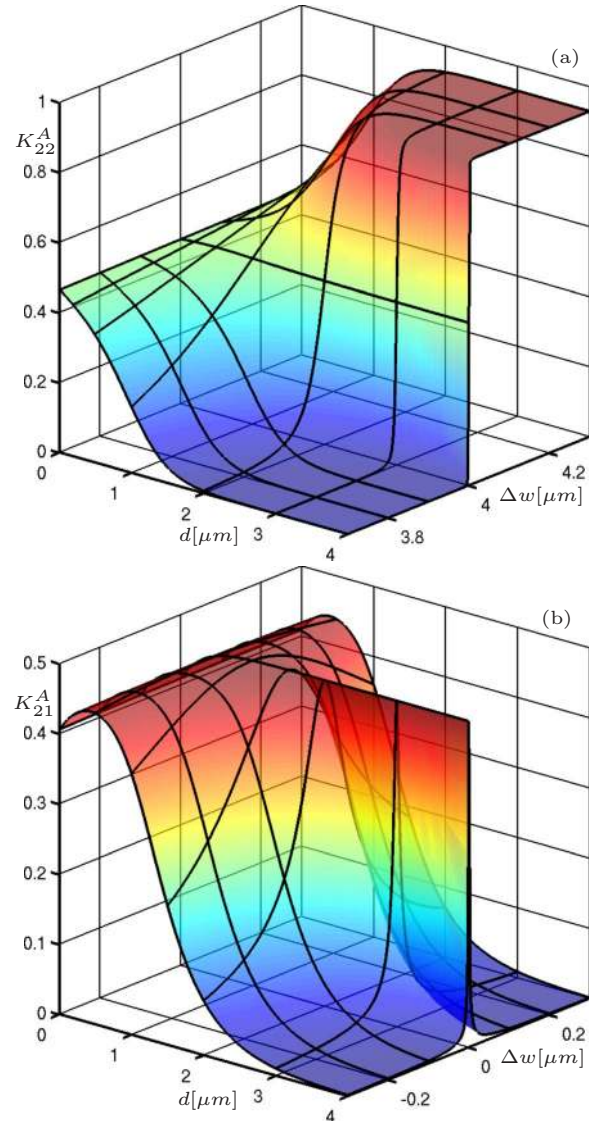
FIG. 5. (Color online) Modal gain coefficient K_{22}^A (a) and composite-mode coupling coefficient K_{21}^A (b) as a function of the half-distance d and the stripe-width difference \Delta w .
