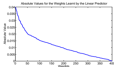
Figure 2: Weights of the linear predictor sorted in descending order in the x-axis according to its absolute value in the y-axis
