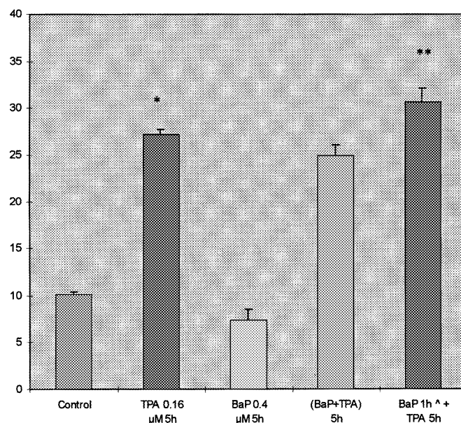
Fig. 3. Superinduction of ODC activity in SHE cells stage-exposed to benzo[a]pyrene and TPA. The four first treatments consisted of 1 h of treatment medium alone (DMEM medium pH 6.7 supplemented with 5% fetal calf serum) then removal and replacement for 5 h with medium alone, 0.16 μM TPA, 0.4 μM BaP or co-treatment (TPA + BaP) respectively. For the fifth treatment BaP 1 h + TPA 5 h = pre-treatment with 0.4 μM BaP for 1 h then removal and replacement with TPA for 5 h. *Result significantly different from control ( P < 0.05 ); **ODC stimulation significantly different from that obtained with TPA alone ( P < 0.05 ). Results are of triplicate determinations and a second experiment yielded similar results.
