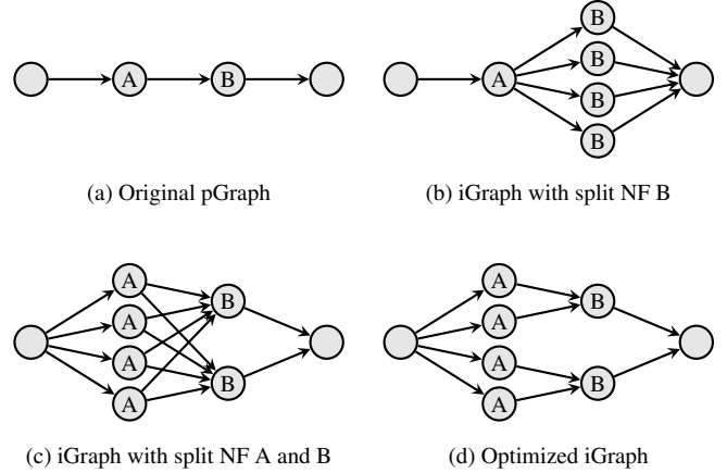
Figure 4: Transformations of a pGraph (a) into an iGraph (b, c, d).
