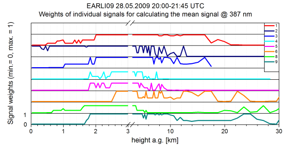
Figure 6: Same as figure 3 but for 28.05.09, without clouds.
