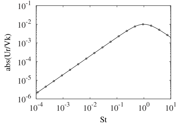
Fig. B.1. Radial velocity of test particles in terms of Keplerian velocity. The points indicate the results of numerical simulations, and the solid line expresses the analytical solution (B.1).
