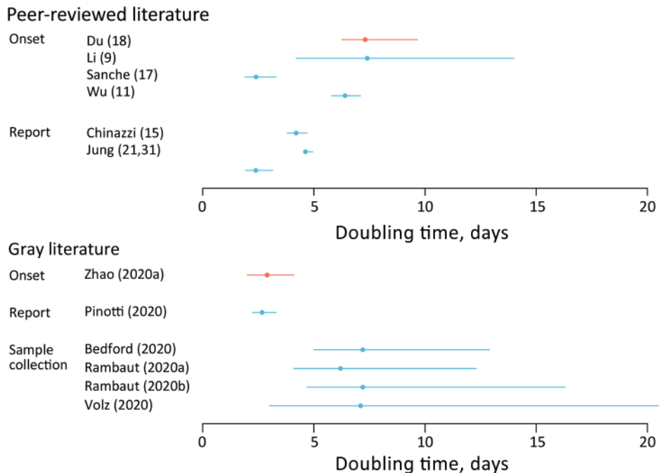
Figure 4. Estimated doubling time for coronavirus disease based on search in peer-reviewed literature and gray literature. Error bars indicate confidence (blue) or credible (red) intervals. Gray literature sources: Onset: Zhao et al., unpub. data, https://www.medrxiv.org/content/10.1101/2020.02.06.20020941v1 ; report: Pinotti et al., unpub. data, https://www.medrxiv.org/content/10.1101/2020.02.24.20027326v1 ; sample collection: Bedford, unpub. data, http://virological.org/t/phylogenetic-estimation-of-incidence-and-prevalence-of-novel-coronavirus-ncov-infections-through-time/391 ; Rambaut, unpub. data, http://virological.org/t/phylogenetic-analysis-176-genomes-6-mar-2020/356 ; Rambaut, unpub. data, http://virological.org/t/phylogenetic-analysis-176-genomes-6-mar-2020/356 (same); Volz et al., https://spiral.imperial.ac.uk/bitstream/10044/1/77169/11/2020-02-15-COVID19-Report-5.pdf (also see Appendix Tables 2, 3).
