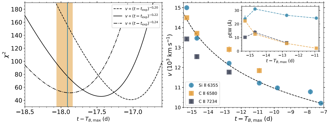
Figure 5. Constraints on t_{\text{exp}} from the velocity evolution of Si II. Left panel: the dashed, solid, and dot-dashed curves show \chi^2 for fitting power laws with indices -0.20 , -0.22 , and -0.24 , respectively. The blue vertical line and the orange shaded region indicate t_0 and its 95% confidence interval from Section 4.1, respectively. Right panel: observed Si II \lambda 6355 velocities (blue circles) and the best-fit power-law model with an index of -0.22 (dashed line). For comparison, the measured velocities of C II \lambda\lambda 6580, 7234 are also shown. Typical uncertainties are smaller than the size of the points. Right inset: evolution of the pseudo-equivalent width of Si II \lambda 6355 and C II \lambda\lambda 6580, 7234 in the \sim 7 days following explosion.
