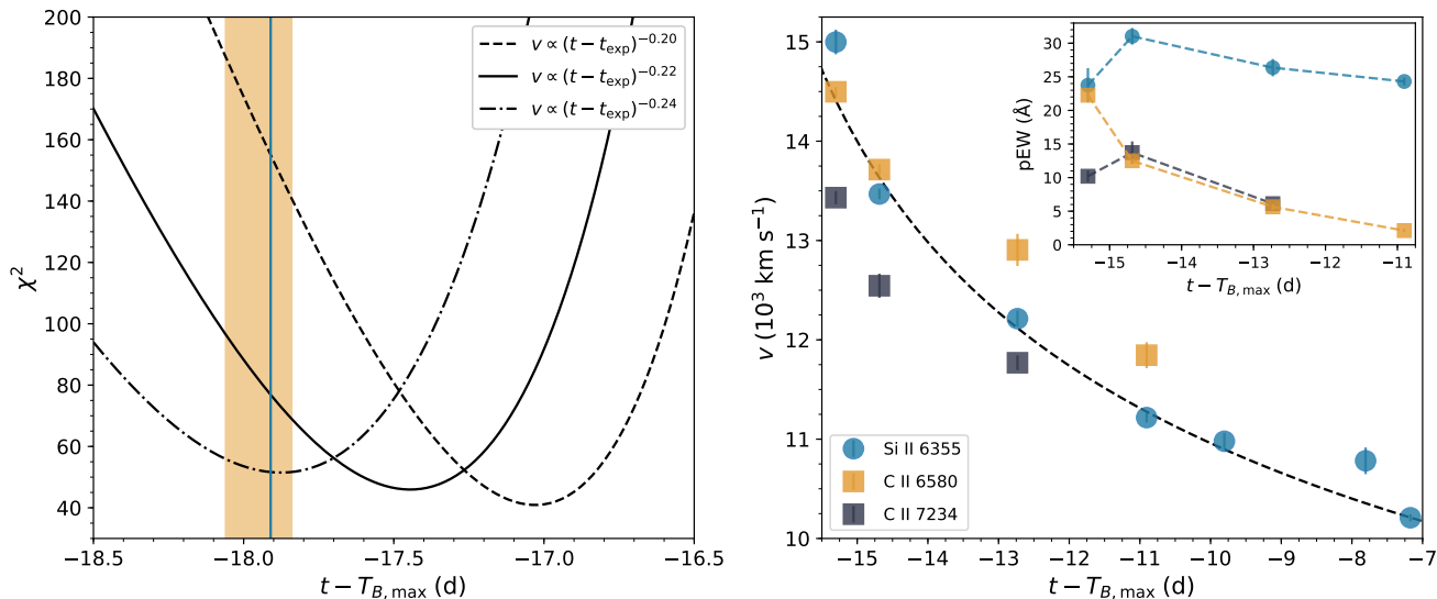
Figure 4. Constraints on t_{\text{exp}} from fitting the velocity evolution of Si II. Left panel: the dashed, solid and dash-dotted curves show \chi^2 for fitting power laws with indices -0.20 , -0.22 and -0.24 , respectively. The blue vertical line and the orange shaded region indicate t_0 and its 95% confidence interval from Section 4.1, respectively. Right panel: Observed Si II \lambda 6355 velocities (blue circles) and the best-fit power-law model with an index of -0.22 (dashed line). Additionally, the measured velocities of C II \lambda\lambda 6580 , 7234 are shown. Typical uncertainties are smaller than the size of the points. Right inset: Evolution of the pseudo-equivalent width of Si II \lambda 6355 , and C II \lambda\lambda 6580 , 7234 in the \sim 7 d following explosion.
