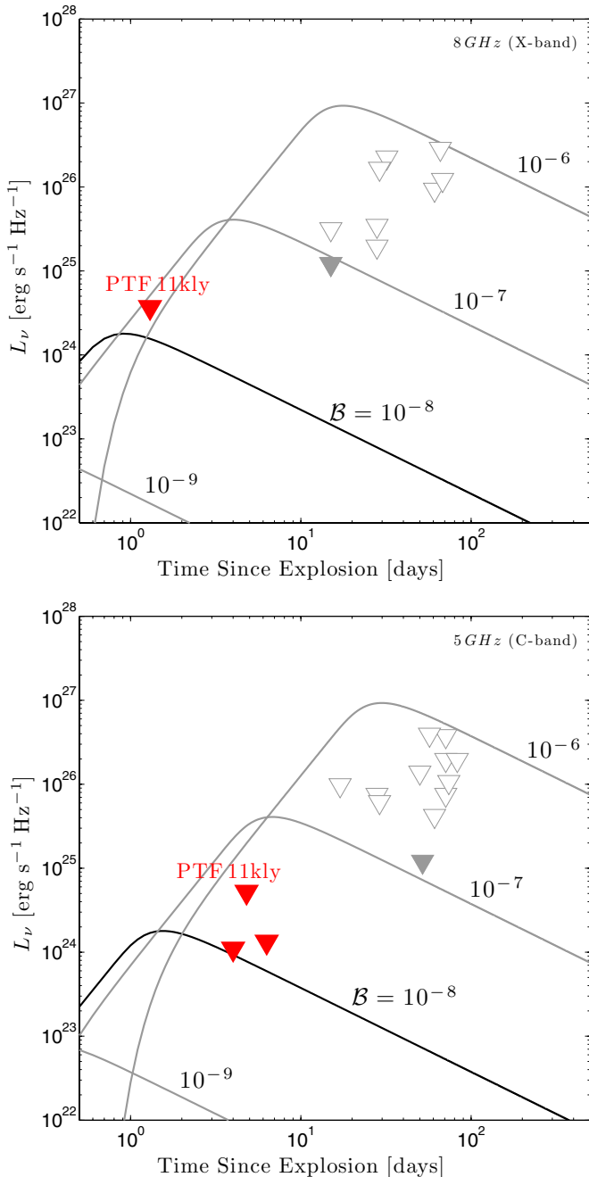
Figure 2. Model light curves for four different values of B = \epsilon \dot{M}/w where \epsilon^2 = \epsilon_B \epsilon_e , w is the wind velocity, and \dot{M} is the mass-loss rate (see also Section 3.1). We assume the following normalization, \epsilon = 0.1 , w = 10^7 \text{ cm s}^{-1} , and v_s = 4 \times 10^9 \text{ cm s}^{-1} . Model light curves for four values of B = [10^{-6}, 10^{-7}, 10^{-8}, 10^{-9}](0.1/\epsilon)w_7 M_\odot \text{ yr}^{-1} are shown. Top panel is for X band (8 GHz) while bottom panel is for C (5 GHz) band. The open triangles in both panels show upper limits from Panagia et al. (2006). The gray triangle in the top panel is the best limit from Panagia et al. (2006) while that in the bottom panel is the upper limit from Hancock et al. (2011). Red triangles are measurements of PTF11kly and presented in Table 1.
