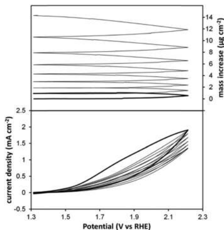
Fig. 2 EQCM experiment wherein the mass balance (top) and current density (bottom) are simultaneously followed as a function of applied potential in the case of a 1 mM solution of 1 in 100 mM Na 2 SO 4 (non-buffered). The first scan is depicted in bold.
