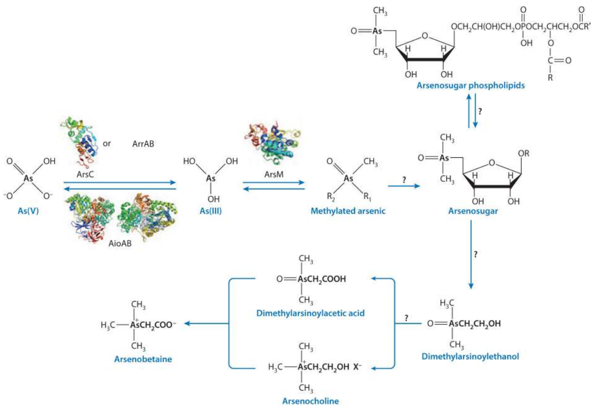
Figure 2. Arsenic species and their biotransformations. Known enzymes for biotransformation are indicated in each step, and representative protein structures are shown for each enzyme: ArsC (Martin et al. 2001), AioAB (Ellis et al. 2001, Warelow et al. 2013), and ArsM (Ajees et al. 2012). Question marks indicate steps for which the molecular mechanism has yet to be unraveled. The diagram is partly adapted from Edmonds & Francesconi (1987).
