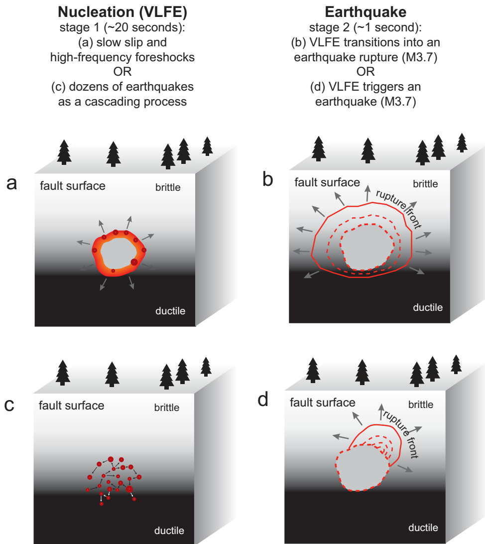
Figure 4: Alternative interpretations for the two stages of nucleation and rupture. Our preferred interpretation for the 2016 event is a \rightarrow b , that the M_w 3.7 earthquake nucleated from a very-low-frequency earthquake (VLFE) associated with slow slip. Alternative interpretations are a \rightarrow d , c \rightarrow b , and c \rightarrow d . The 2015 VLFE event comprised stage 1 (a or c) but did not transition into an earthquake.
