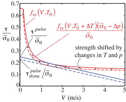
Figure 3. \tau_{dyn}^{pulse} was defined in a similar way to Zheng and Rice [1998] after taking into account changes in T and p due to thermal pressurization during the nucleation process. Steady state strength is decreased due to an increase in T , which decreases V_w(T) and hence f_{ss}(V, T) , and an increase in p , which decreases \bar{\sigma} .
