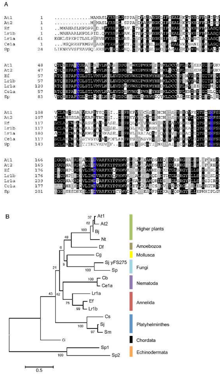
Figure 3. Earthworm phytochelatin synthase sequences compared to phytochelatin synthase sequences from other species. A: alignment of Lumbricus rubellus phytochelatin synthase sequences (conserved N-terminal region only, full sequence shown in Figure S1) against key species with validated PCS activity ( Arabidopsis thaliana PCS1 and PCS2, Eisenia fetida , L. rubellus PCS1a and PCS1b, Caenorhabditis elegans , and Schizosaccharomyces pombe ). Conserved residues are shown with white text on black background; the conserved Cys-His-Asp catalytic triad is shown with yellow on blue background. B: Phylogenetic tree of phytochelatin synthase genes. The evolutionary history was inferred by using the Maximum Likelihood method based on the Whelan and Goldman model [48]. The tree with the highest log likelihood (-3323.4018) is shown. The percentage of trees in which the associated taxa clustered together is shown next to the branches. Initial tree(s) for the heuristic search were obtained by applying the Neighbor-Joining method to a matrix of pairwise distances estimated using a JTT model. A discrete Gamma distribution was used to model evolutionary rate differences among sites (5 categories (+G, parameter = 1.9794)). The tree is drawn to scale, with branch lengths measured in the number of substitutions per site. The analysis involved 19 amino acid sequences. All positions containing gaps and missing data were eliminated. There were a total of 126 positions in the final dataset. Evolutionary analyses were conducted in MEGA5 [49]. At – A. thaliana . Bj – Brassica juncea . Nt – Nicotiana tabacum . Df – Dictyostelium fasciculatum . Cg – Crassostrea gigas . Sj yFS275 – Schizosaccharomyces japonicum . Sp – S. pombe . Cb – C. briggsae . Ce1a – C. elegans . Lr1a and Lr1b – Lumbricus rubellus PCs 1a and 1b respectively. Cs – Clonorchis sinensis . Sj – Schistosoma japonicum . Sm – Schistosoma mansoni . Ci – Ciona intestinalis . Sp1 and Sp2 – Strongylocentrotus purpuratus .
