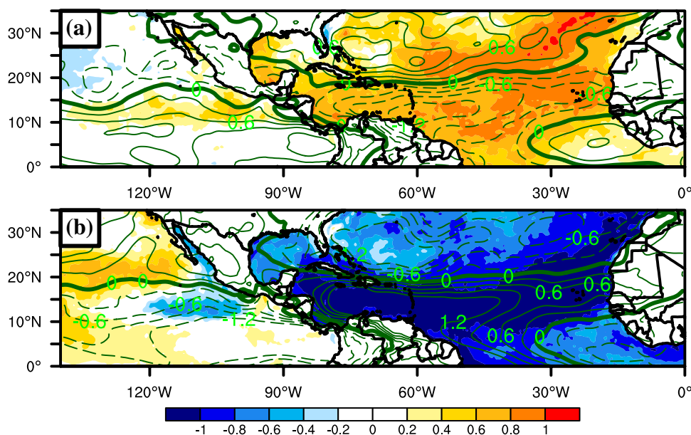
Fig. 8 Standardized anomalies of sea surface temperature (°C, shaded) and anomalies of vertical wind shear (m/s, green contours) for a years when their AMO index was in the upper tercile and b years when their AMO index was in the lower tercile. Dashed green lines represent negative anomalies of wind shear, the bold line represents the value of zero and the continuous green lines represent positive anomalies
