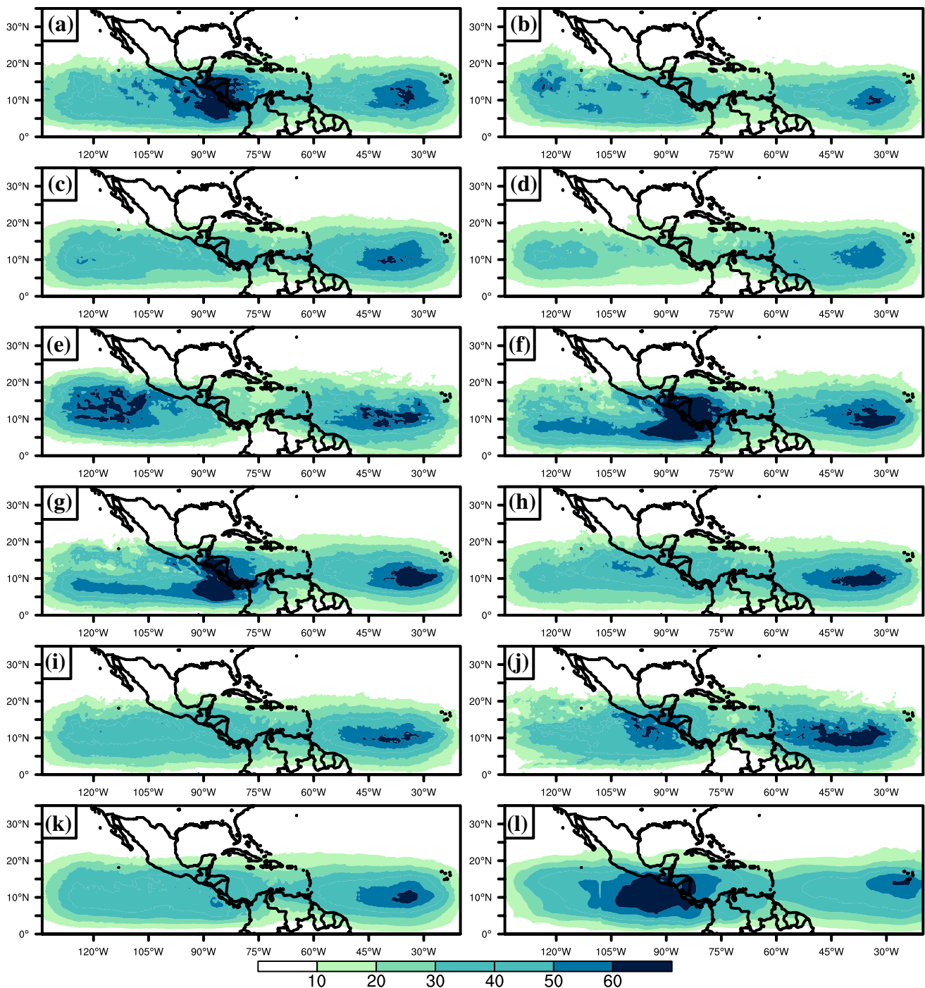
Fig. 13 As Fig. 12 but for the contribution (%) of easterly waves to summer rainfall
