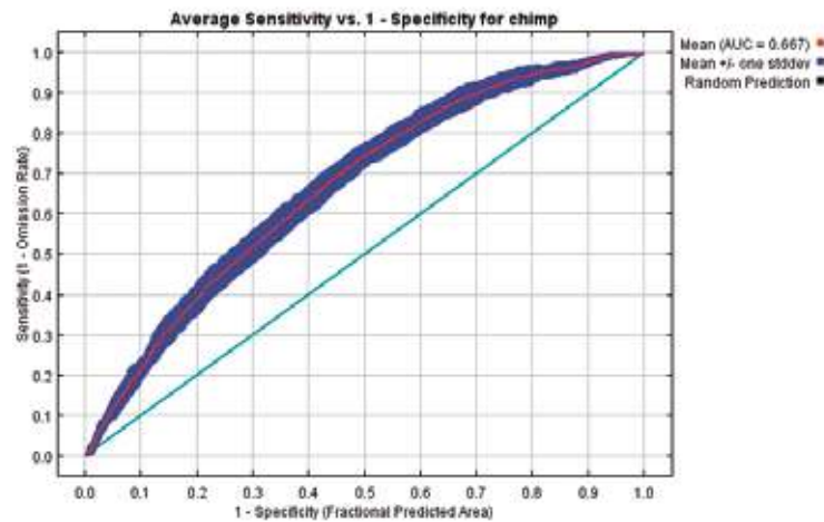
Figure 4.2. ROC curve for the 4-variable model with blue \pm one standard deviation shading. It can be seen that the curve is significantly better than a random prediction (straight line).
