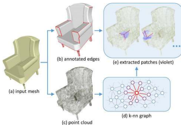
Fig. 4: Procedure to extract patches (a local group of points) from a point cloud; note that (a) and (b) are available only in the training (but not inference) phase.
