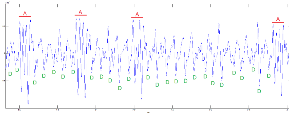
Figure 11: Extracted DA-sequence obtained from iPhone 3GS during an OpenSSL secp256k1 signature operation. The leakage was measured using the Tracker Pre sound card and the improvised EM probe. The DOUBLE and ADD operations can clearly be seen.
