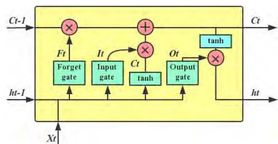
FIGURE 3. Typical structure of a LSTM unit.
