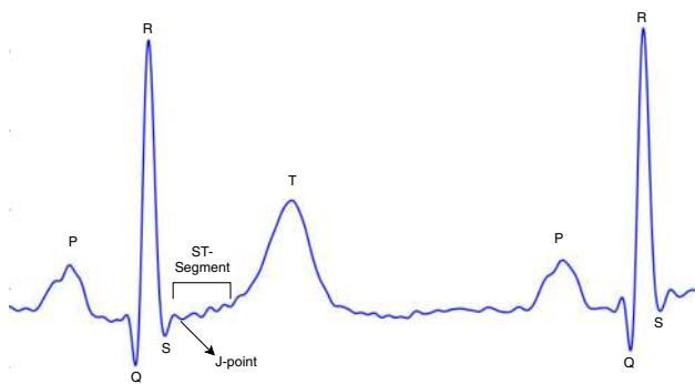
Fig. 1 ECG intervals and reference points during a cardiac cycle (one channel/lead)
