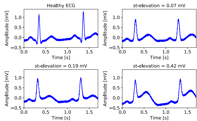
Fig. 2 Surrogate signals with several ST-elevation levels
