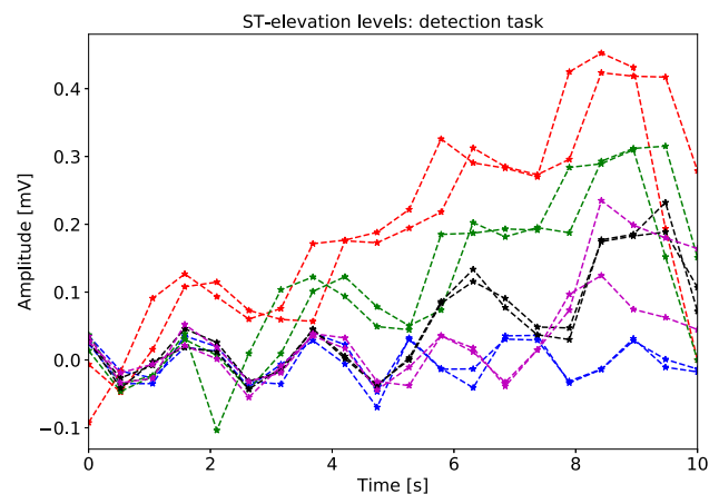
Fig. 5 ST-elevation levels of ECG files used in detection task
