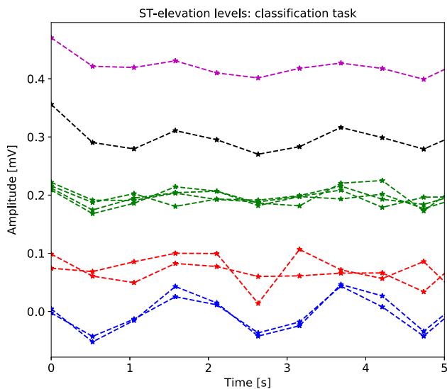
Fig. 6 ST-elevation levels of ECG files used in classification task
