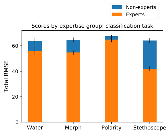
Fig. 12 Bar plot experts/non-experts classification task task
