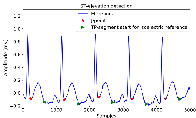
Fig. 4 ST-elevation detection
