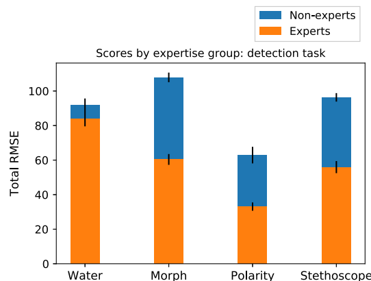
Fig. 11 Bar plot experts/non-experts detection task
