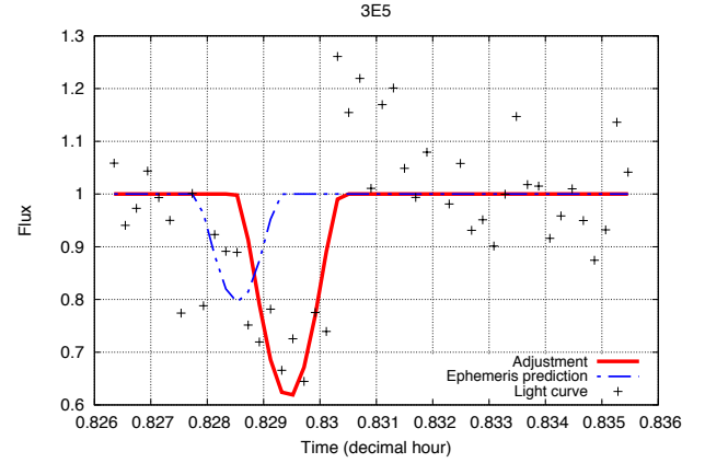
Fig. 5. Fitted light curve (flux versus time in decimal hour) of the 3E5 event. Ganymede eclipses Amalthea on 2015 Apr. 7. The blue dot-dash line denotes the theoretical flux drop according to JUP310 ephemeris (Jacobson 2013); the red line denotes the fitted flux drop of the event.
