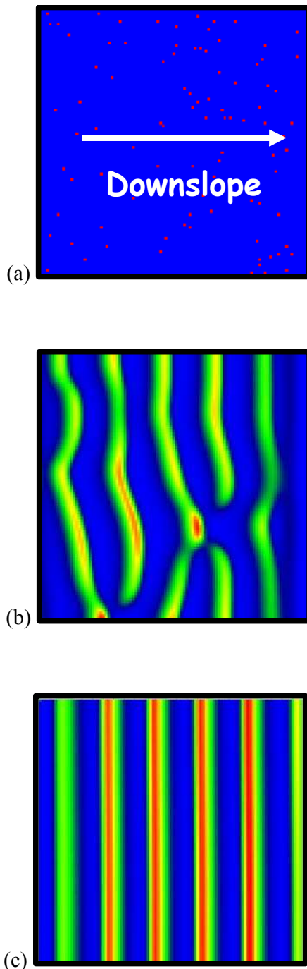
Fig. 3. Self-organization of vegetation into a banded pattern for a planar hillslope with sheet flow. The scale is 200\text{ m} \times 200\text{ m} on a slope of 1.4\% . (a) Initial conditions of random plant peaks in 1\% of the grid elements, (b) Vegetation pattern for t=2560 days, (c) Stationary bands have completely developed for t=15 years.
