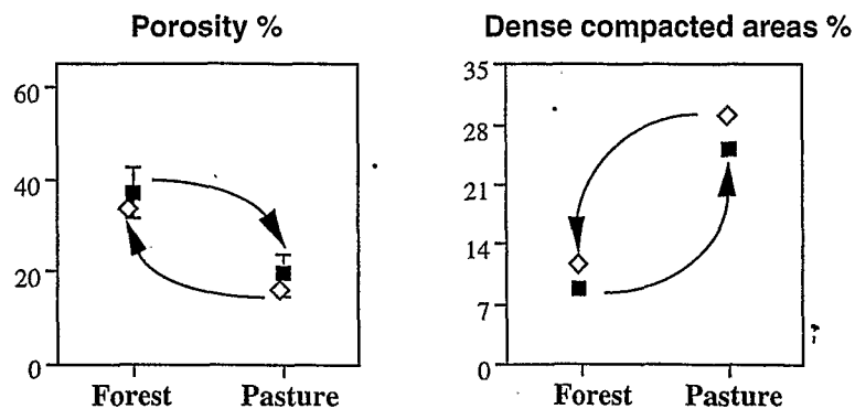
Fig. 3. Changes in the proportions of soil porosity and dense areas (identified as earthworm casts) measured on thin sections of soil in monoliths ( 25 \times 25 \times 30 cm) 1 year after their transplantation from a forest with a diverse soil macrofauna to a pasture invaded by the endogenic earthworm, Pontoscolex corethrus (□), and vice versa (◇) (Barros, 1999).
