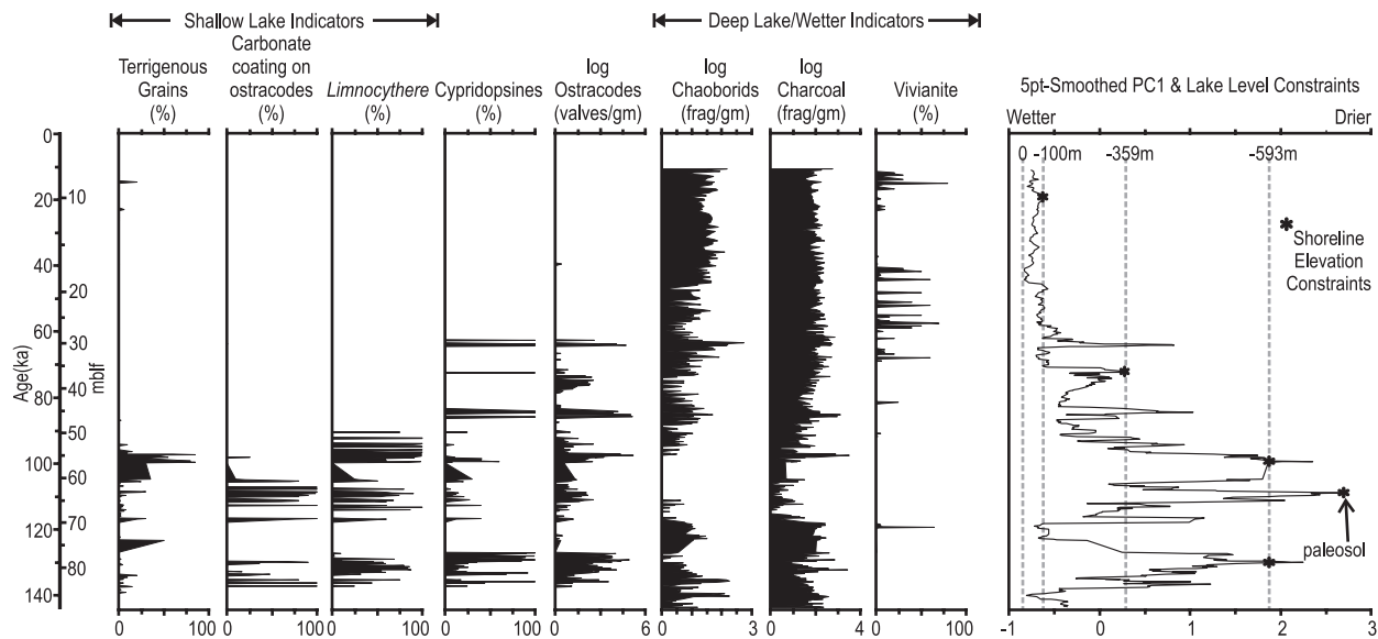
Fig. 1. Screen-wash records vs. time and depth for core 1C and PCA first axis of variance (strongly correlated with lake level) vs. time and depth. mbf, meters below lake floor. The probable paleosol at 108.5 ka indicates a minimum lake-level decline: The lake may have dropped below the core site elevation.
