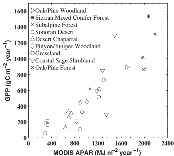
Figure 2 Annual gross primary production (GPP; \text{gC m}^{-2} \text{year}^{-1} ) calculated by integrated eddy covariance as a function of the contemporaneous absorbed photosynthetically active radiation (APAR; \text{MJ m}^{-2} \text{year}^{-1} ) based on Moderate Resolution Imaging Spectroradiometer (MODIS) observations. The eddy covariance observations were made at 10 sites in southern California and the Sierra Nevada (see Table S1 and Goulден et al. , 2012 for site details).
