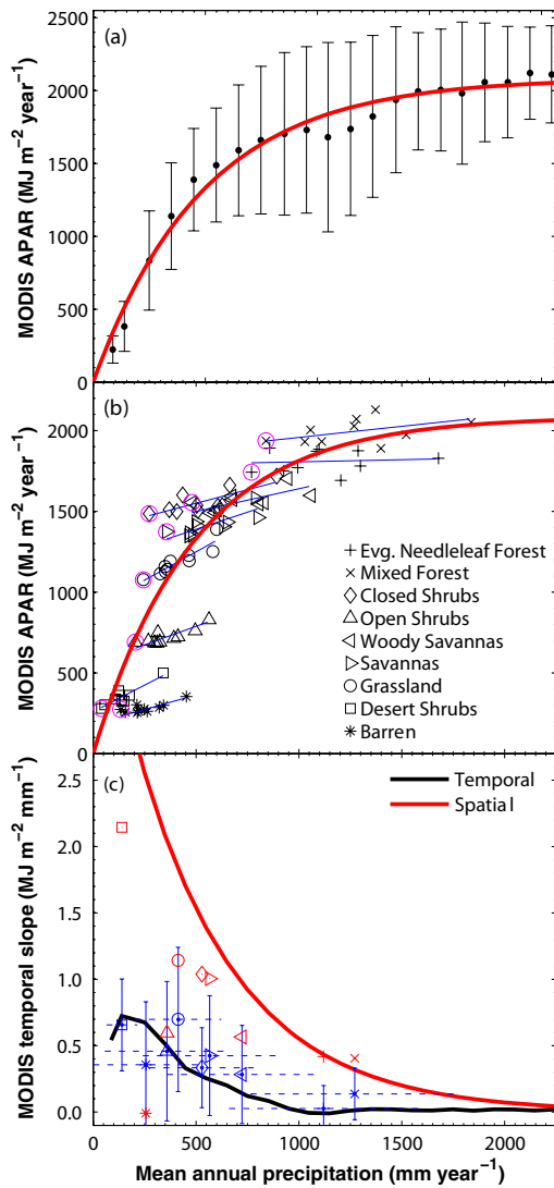
Figure 3 Annual Moderate Resolution Imaging Spectroradiometer (MODIS) absorbed photosynthetically active radiation (APAR; MJ m -2 year -1 ) (a, b) and the slopes of the relationship between MODIS APAR and precipitation (MAP; mm year -1 ; 2001–10 mean) across California. APAR was averaged (a) during 2001–10 for MAP bins at 100 mm year -1 intervals, and (b) averaged within each year over each dominant land-cover type. The solid red lines in (a) and (b) show the overall fit between mean APAR and MAP across California, and in (c) the slope of the regression between mean APAR and MAP across the entire state (e.g. the derivative of the red line in a). The solid blue lines in (b) show the least squares regression for each land-cover type; the slopes of these lines provide a measure of the sensitivity of APAR to interannual precipitation variation within each cover type. The circled magenta symbols in (b) show the average APAR for each land-cover type during the driest observation year. In panel (c), the slope of the interannual APAR versus precipitation relationship was averaged across all pixels in 100 mm year -1 wide MAP bins (solid black line), and summarized for the dominant land covers (blue symbols and lines for mean and standard deviation); the red symbols represent the spatial slope within each land-cover type.
