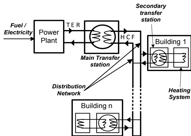
Figure 1. Schematic representation of a district heating network.
