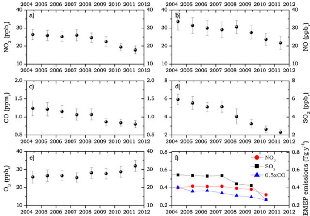
Figure 2. Annual means of air pollutants in Athens. First, second, third, fourth, and fifth panel depict the annual averages of the ground-based measurements of NO 2 , NO, CO, SO 2 , O 3 , respectively. Black thin lines denote the annual standard deviations. Sixth panel presents the official EMEP emissions of NO x (as NO 2 emissions, red circles), SO x (as SO 2 emissions, black squares) and CO (blue triangles) over Greece.
