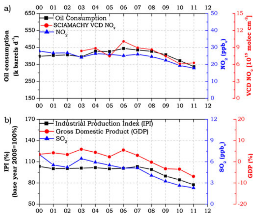
Figure 3. The top row (a) presents the annual means of nitrogen dioxide levels (NO 2 ) over Athens (blue) compared to the tropospheric SCIAMACHY VCD NO 2 (red) and the oil consumption per day (black). The bottom row (b) depicts the annual means of sulfur dioxide (SO 2 ) levels in Athens (blue), the Gross Domestic Product of Greece (red) and the Industrial Production Index, IPI (black).
