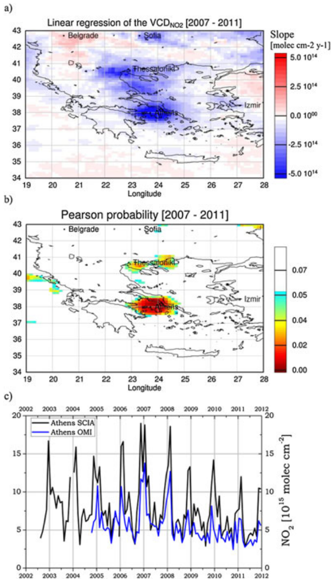
Figure 1. (top row) Linear regression of the annual averages of the nitrogen dioxide vertical columns retrieved for the period 2007–2011. Red color denotes an increase and blue a decrease in VCD NO 2 values. Middle row presents the Pearson probability of the linear regression; dark red color denotes statistical significant linear correlations ( a < 0.05 ). Bottom row depicts the monthly mean averages of the NO 2 vertical column densities over Athens [23.750 ± 0.125E, 38.000 ± 0.125 N] derived using the SCIAMACHY (black line) and the OMI (blue line) data.
