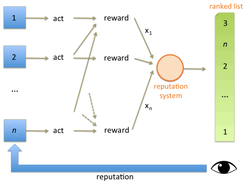
Figure 5: In a reputation system for a multi-agent AI, each agent chooses an action, and the combined effect of these actions generates rewards (i.e., utility). Based on the actions taken and rewards received, agent i can submit a report, x_i to the reputation system. The reputation system aggregates this feedback, for example providing a ranked list to reflect the estimated trustworthiness of agents. Each agent observes this ranked list, and this information may influence future actions.
