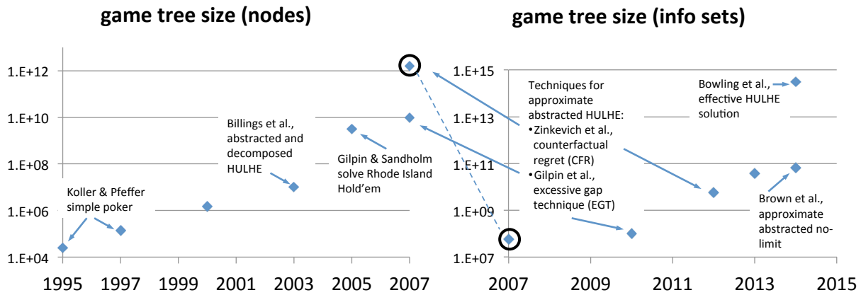
Figure 2: Researchers produced steady exponential progress on solving games of imperfect information from 1995 to the present. Up to 2007 (left), game size was generally reported in terms of nodes in the game tree. Based on methods introduced around that time, it became more meaningful (right) to report size in terms of the number of information sets (each many nodes), which represent distinct situations as perceived from the perspective of a player. The circled data points correspond to the same milestone; combining the two graphs thus demonstrates the continual exponential improvement.
