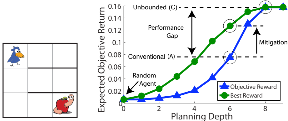
Figure 1: A bounded reinforcement learning agent performs better by pursuing a designed reward function different from the objective reward : its actual fitness evaluation. Results (right) from a gridworld foraging domain (left), for various limits on the agent’s planning horizon (16). Unless the agent is perfectly rational (i.e., no horizon limit)—not typically feasible in realistic applications—the designer can often achieve better fitness by directing the agent to optimize an alternative measure.
