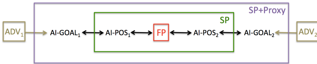
Figure 4: Two generations of sponsored search mechanisms. Early designs were first price (FP) and advertisers (ADV) used AIs (AI-POS) to maintain a position on the list of search results at the lowest possible price. Second price (SP) auction mechanisms were introduced, designed to replace the combination of FP and AI-POS. Advertisers adopted new AIs (AI-GOAL) to achieve higher-level goals such as maximize profit or maximize the number of clicks. The second price auction was extended to include proxy agents (SP+Proxy), designed to replace the combination of SP and AI-GOAL.
