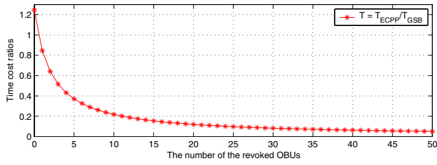
Fig. 6. Time efficiency ratio T_{EG} = T_{ECPP}/T_{GSB} with a number of n revoked OBUs, where n is ranged from 1 to 50.
