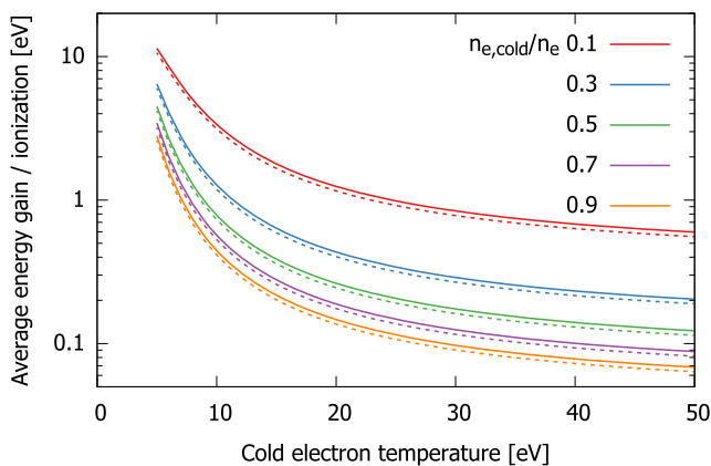
FIG. 7. The calculated average energy gain of the Ar^+ ion ionized via electron impact or charge exchange ionization as a function of the cold electron temperature at different cold electron fractions. The charge state distribution of the confined ions was taken either from afterglow peak currents (solid) or from continuously extracted currents (dashed).
