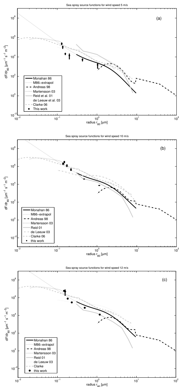
Fig. 6. Comparison of results from this work with a few sea spray source functions available in the literature for a number of different wind speeds (a) 5 \text{m s}^{-1} , (b) 10 \text{m s}^{-1} , (c) 12 \text{m s}^{-1} .
