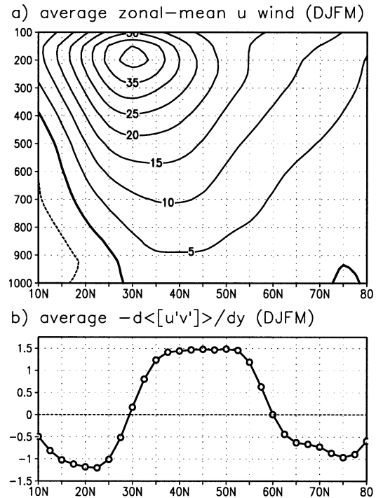
FIG. 2. (a) Time- and zonal-mean zonal wind (DJFM). (b) Time-, vertical-, and zonal-mean eddy momentum flux convergence in \text{m s}^{-2} day ^{-1} . Spherical effects are taken into account.
