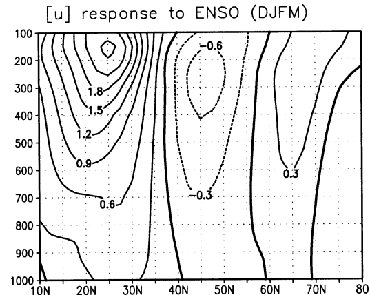
FIG. 1. Zonal-mean zonal wind regressed on monthly ENSO time series (DJFM).
