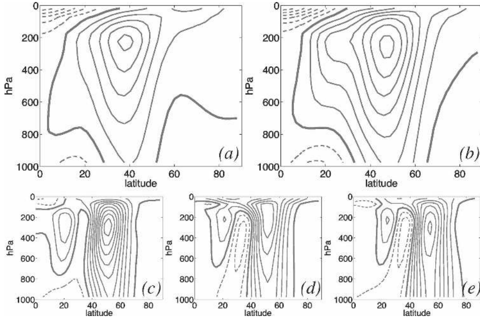
FIG. 1. (a),(b) The time and zonal average zonal wind for two simulations from experiment set I. In (a), \Delta T_{eq} = 40 K and in (b), \Delta T_{eq} = 80 K. (c)–(e) The difference in the time and zonal average zonal winds between two simulations. Panel (c) shows the difference between the simulations shown in (b) and (a), in which the equilibrium temperature gradient was varied. Panel (d) shows show the difference between two simulations in experiment set III, where the thermal damping was varied: the winds with k_a = 30^{-1} less those in a simulation with k_a = 60^{-1} . Panel (e) shows the difference in winds from two simulations in IV, where the momentum damping was varied: a simulation with k_f = 1.5^{-1} less those in one with k_f = 0.75^{-1} . The contour interval is 5 \text{ m s}^{-1} in (a) and (b) and 2.5 \text{ m s}^{-1} in (c)–(e). Negative contours are dashed and the zero contour is doubled in thickness.
