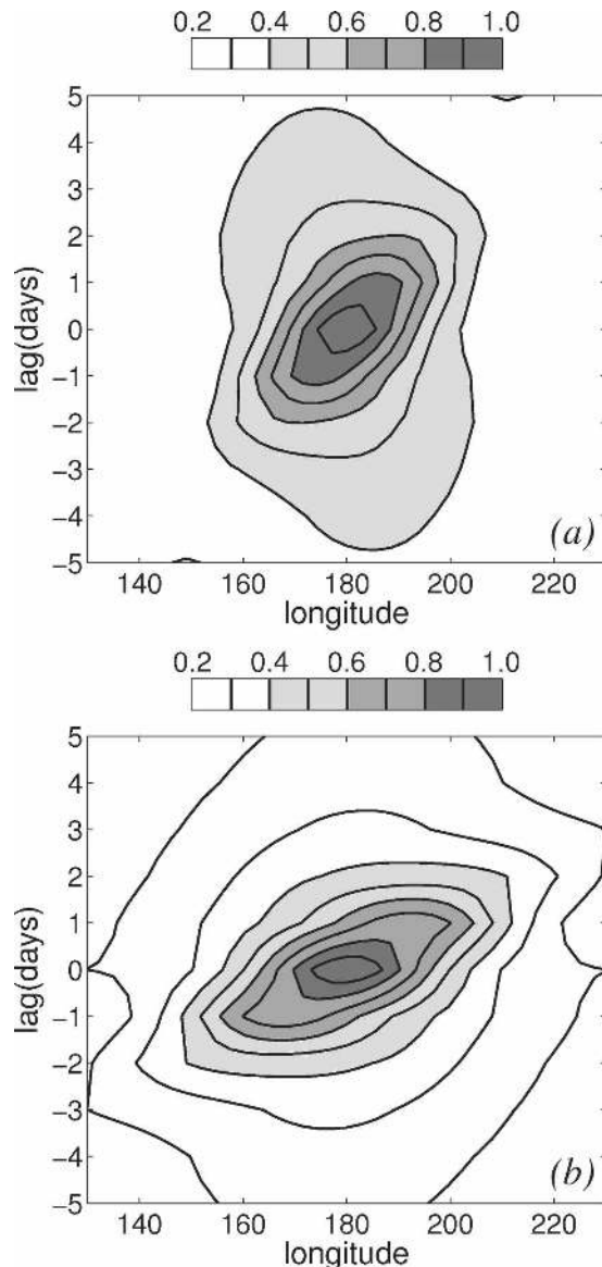
FIG. 7. The lag–longitude autocorrelation of the dipole index, D_f(t, \lambda) , for the simulations with (a) \Delta T_{\text{eq}} = 40 and (b) \Delta T_{\text{eq}} = 80 K. The base longitude for the map is 180^\circ . As noted in the text, the correlation maps at other longitudes are the same with respect to the base point, except for sampling errors. We thus averaged over all longitudes to improve statistics, and the choice of this particular base point was made for plotting purposes.
