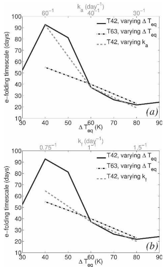
FIG. 2. (a), (b) The e -folding time scale of the zonal index as function of model parameters. The solid and dot-dashed black curves illustrate the e -folding time scale as function of \Delta T_{\text{eq}} , and correspond with the lower x axis. The dashed gray curve in (a) marks the e -folding time scale as a function of k_a and in (b) the time scale as a function of k_f . In both cases the values of the damping coefficients are shown on the upper x axis. In each sensitivity test the other parameters were held constant at their control values, as listed in Table 1.
