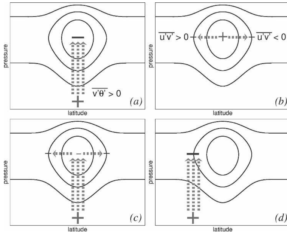
FIG. 11. A diagram of the eddy-mean flow feedback. Solid contours mark the position of the zonal mean winds. Dashed arrows denote the propagation of wave activity, or, equivalently, the direction of EP fluxes. Plus and minus signs indicate divergence and convergence of the EP fluxes, and so westerly or easterly torque on the mean flow. (a), (b) The impact of eddy heat and momentum fluxes on an eddy formed in the jet core is broken down, leading to (c) the net forcing of the flow. Momentum fluxes in upper levels spread the easterly torque over the jet, maintaining the shear in the core. (d) For an eddy generated on the flank of the jet, weak upper-level winds limit meridional propagation, and the shear tends to be reduced only locally.
