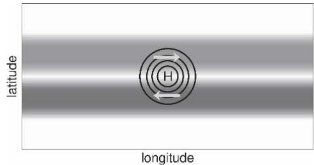
FIG. 8. A cartoon illustrating the potential for a single eddy to project strongly on the zonal index, or annular mode. The dipole structure of the surface zonal wind is illustrated with positive and negative bands, and the eddy marked by black contours of pressure.
