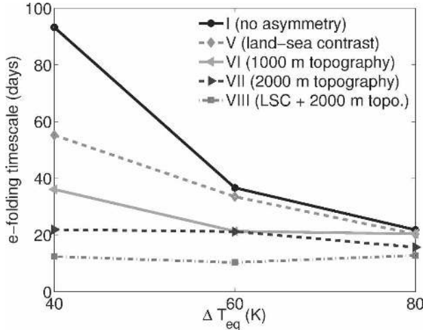
FIG. 3. The impact of zonally asymmetric forcing and the equilibrium temperature gradient on the e -folding time scale of the annular mode. For experiment sets I and V–VIII, we plot the e -folding time scale of the first EOF of SLP in three simulations with different values of \Delta T_{\text{eq}} , the equilibrium temperature gradient. In the zonally symmetric simulations of I the first EOF has a perfectly annular structure. With increased zonal asymmetry, in particular the simulations in VIII (where LSC refers to land–sea contrast), the annular mode has an NAO-like zonal structure, with most emphasis in the exit region of the storm track.
