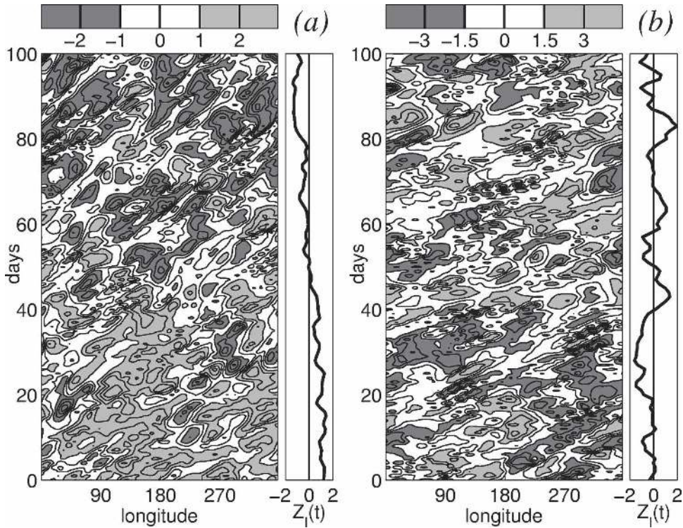
FIG. 6. Hövmöller diagrams of the dipole index D_I(t, \lambda) for simulations with (a) \Delta T_{eq} = 40 and (b) 80 K. The contour interval is (a) 1 and (b) 1.5 deviations. The curves on the right show the behavior of the zonal index as a function of time, in units of standard deviations.
