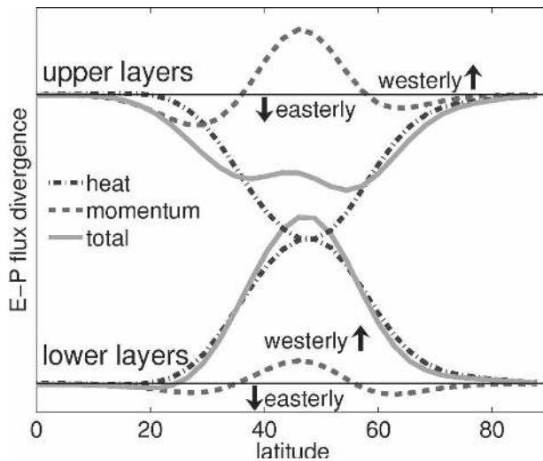
FIG. 12. The acceleration of the mean flow, \partial\bar{u}/\partial t , by the 2–10-day bandpass eddies in the control simulation, averaged over all times when the zonal index is neutral, |Z_i(t)| < 1 . The upper curves show the forcing averaged over the top 500 hPa of the atmosphere, the lower curves the same for the bottom half of the atmosphere. The dashed curves show the acceleration due to eddy momentum fluxes, -r_0^{-1}(\partial_0\bar{u}'v' - 2 \tan\theta\bar{u}'v') , and the dot-dashed curves that are due to eddy heat fluxes, f\partial_p(\bar{v}'\theta'/\theta_p) . The solid curves show the total acceleration, the sum of the two other curves.
