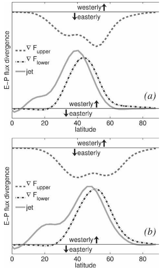
FIG. 13. Evidence for the eddy-mean flow interaction in the control simulation. Composites based on (a) weak and (b) strong zonal index events, as determined by a threshold of \pm 1 std dev of the zonal index Z_i(t) . The dot-dashed curves show the acceleration of the zonal average flow, \nabla\mathbf{F} , by 2–10-day bandpass eddies averaged over the lower half of the atmosphere. The torque is westerly at nearly all latitudes. The dashed curves show the acceleration of the upper half of the atmosphere; a negative (easterly) torque. The solid curves show composites of the upper-level jet: \bar{u} averaged over the upper half of the atmosphere.
