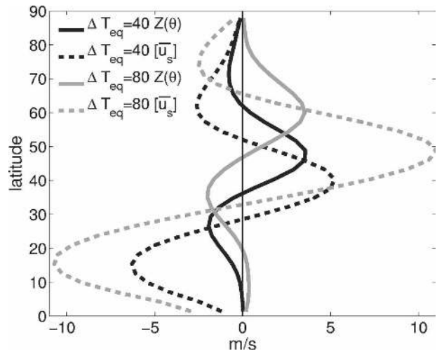
FIG. 5. The time and zonal average surface ( \sigma = 0.975 ) winds, [\bar{u}_s] , and the first EOF of \bar{u}_s , Z(\theta) , for simulations for experiment I with \Delta T_{\text{eq}} = 40 and 80 K. Units for the EOF patterns are per standard deviation of their respective zonal indices.
