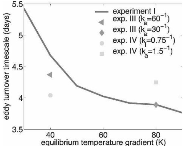
FIG. 4. The eddy turnover time scale, L/K^{1/2} , as a function of the equilibrium temperature gradient, \Delta T_{\text{eq}} . The eddy kinetic energy, K , increases linearly with the equilibrium gradient, while the eddy length scale is roughly constant. Hence the curve is proportional to \Delta T_{\text{eq}}^{-1/2} . Values for four other zonally symmetric simulations in experiments III and IV (where k_a and k_f were varied, respectively) are shown for comparison. The points were plotted near the simulation from experiment I that had the most similar climatology and intraseasonal variability.
