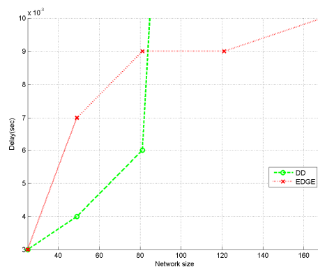
(b) End-to-end delay with different network sizes
