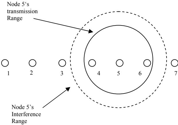
Figure 1: Transmission and interference range for a chain of nodes. Nodes within 3 hops interfere with each other.
