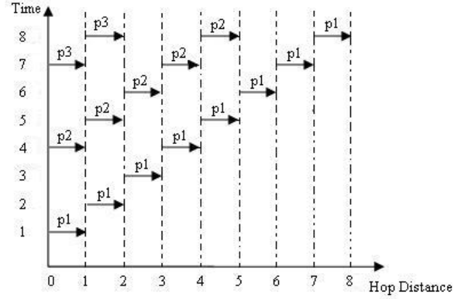
Figure 2: Pipelining mechanism of data transmission in sensor networks with intra-flow interference taken into account.
