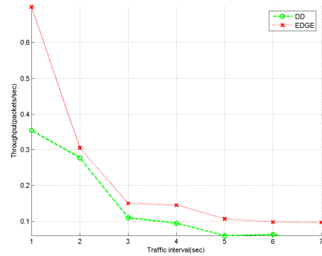
(a) Throughput with different traffic rates.
