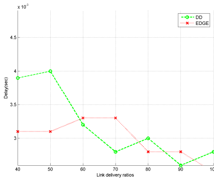
(b) End-to-end delay with different delivery ratios of lossy links.
