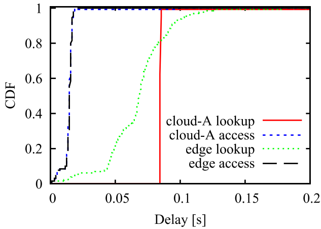
Fig. 14: Metro scenario – 60 GWs - Rate 100 [req/s].
