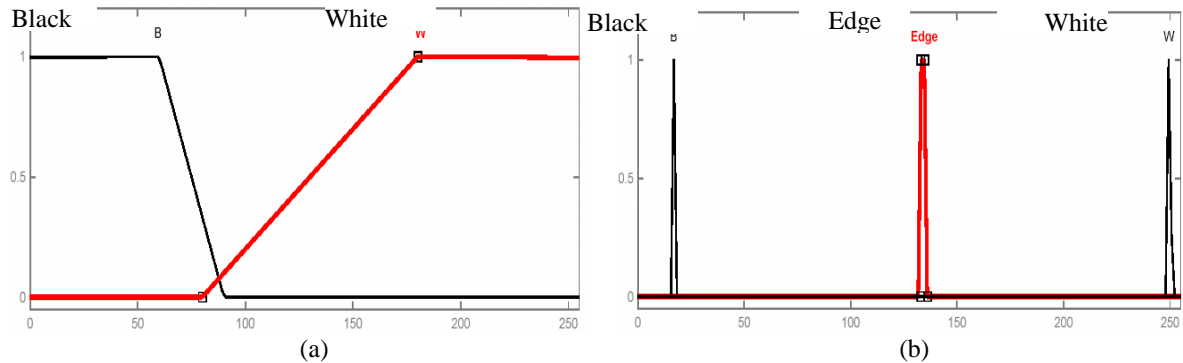
Fig. 3 Membership functions of the fuzzy sets associated to the input and to the output
