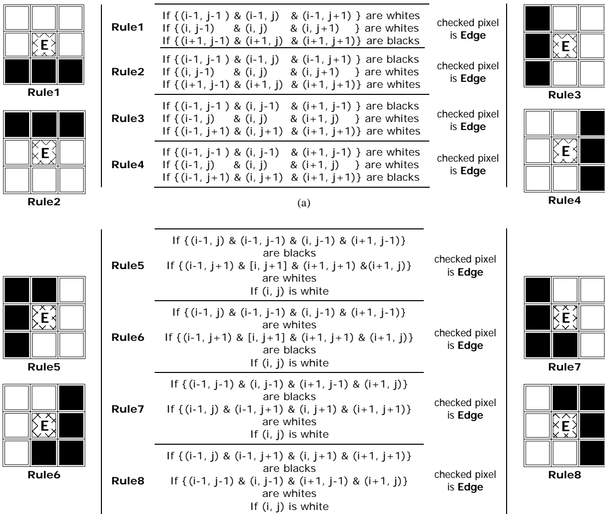
(b) Fig. 4 The Fuzzy System rules
