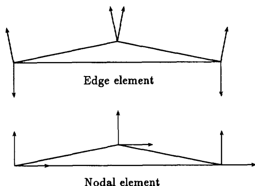
Fig. 4. Extremely flat triangular elements (2D) with bases of local coordinate systems
