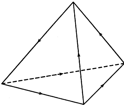
Fig. 2. Mixed "linear" edge element (Whitney 1)
