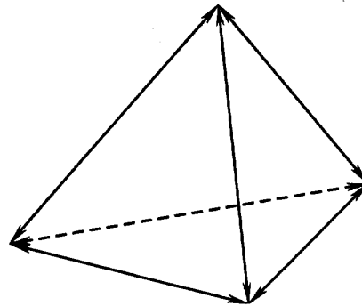
Fig. 3. Consistently linear edge element
