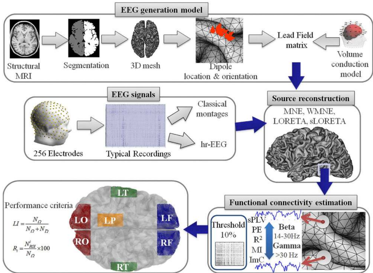
Figure 1. The different steps of the comparative study. hr-EEG: high-resolution EEG, MNE : Minimum norm estimate, wMNE : Weighted Minimum norm estimate, LORETA : Low resolution Brain Electromagnetic Tomography, sLORETA : Standardized Low resolution Brain Electromagnetic Tomography, sPLV : single-trial Phase Locking Value, PE : Phase Entropy, R 2 : linear correlation coefficient, MI : Mutual Information, ImC : Imaginary Coherence ROIs : Regions of Interest, LO : Left Occipital; RO : Right Occipital, LT : Left Temporal, RT : Right Temporal, LF : Left Frontal, RF : Right Frontal, LP : Left Parietal. doi:10.1371/journal.pone.0105041.g001
