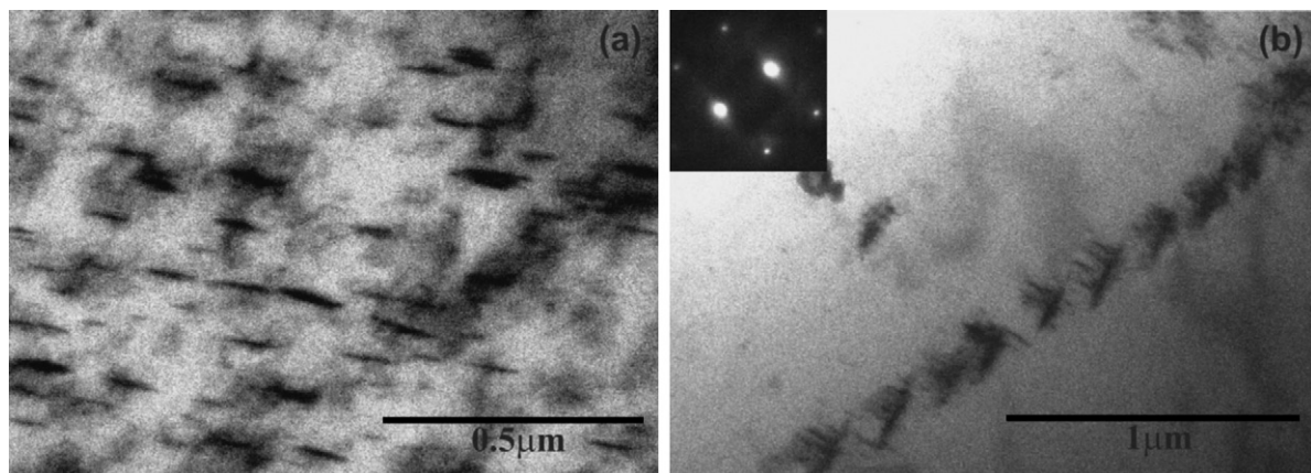
Fig. 3. (a) Needle like precipitates observed in the ferritic phase of DSS grade DIN W Nr. 1.4462 after aging treatment at 475 °C for 100 h; (b) same grain observed in g = (0 \bar{1} 1) diffraction condition [56].
