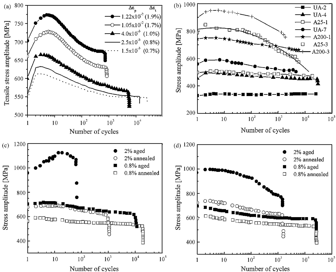
Fig. 9. Cyclic hardening/softening curves for DSS grades (a) SAF 2507 at different plastic strain ranges [70]; (b) (f) AISI 329 unaged (UA) and aged (A25, A200) condition [36]; (c) UR52N+ in the annealed and aged condition [42]; (d) B6A920 in the annealed and aged condition [42]. Fig. 9a–d is reprinted with kind permission from Elsevier.
