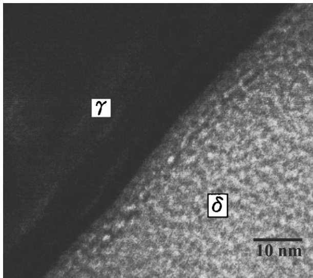
Fig. 4. Modulated contrast observed in the ferritic phase of DSS grade 2205 aged at 475 °C for 2 h. Reprinted with kind permission from Elsevier from [48].
