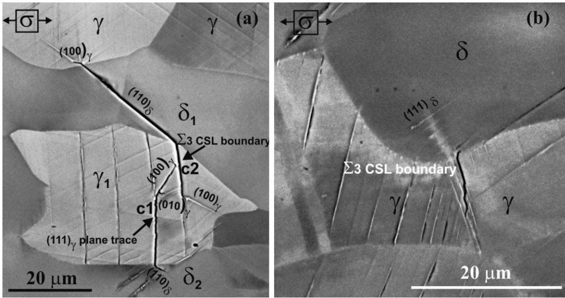
Fig. 11. Fatigue crack initiation in a DSS grade DIN W Nr. 1.4462 aged at 475 °C for 100 h. (a) The growth of crack c2 observed after N=27,000 cycles at \Delta\sigma/2=400 MPa; (b) crack initiation at \Sigma 3 CSL boundary at \Delta\sigma/2=500 MPa [56].
