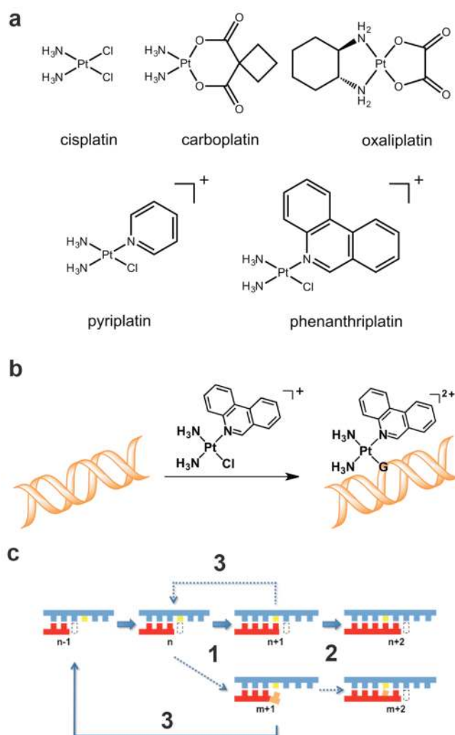
Figure 1. Monofunctional phenanthriplatin-DNA adduct formation and three key fidelity checkpoint steps of Pol II elongation. (a) Structures of platinum-based anticancer compounds. (b) Phenanthriplatin binds guanosine (G) to form a monofunctional platinum-DNA adduct. Double-stranded DNA is shown in orange. (c) Three key fidelity checkpoint steps of Pol II elongation: (1) nucleotide selection and incorporation, (2) RNA transcript extension, and (3) proofreading. DNA and RNA strands in the Pol II elongation complex are shown in blue and red, respectively. Matched (n) and mismatched (m) nucleotides and their template base are shown in red, orange, and yellow, respectively. Correct and incorrect nucleotide incorporations are depicted with n and m, respectively. The position of the next nucleotide to be added is shown with a dotted box. The widths of the solid lines and arrows correspond to the reaction rates; dotted lines indicate very slow reactions.
