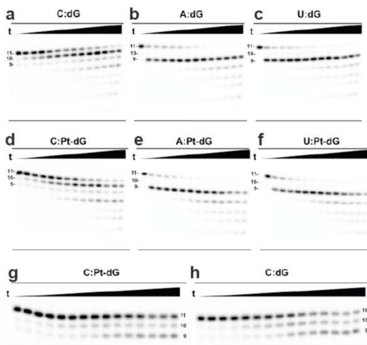
Figure 7. Phenanthriplatin-DNA adducts do not change Pol II proofreading activity in the third step. TFIIS-mediated RNA transcript cleavage from scaffolds containing a pair of (a) C:dG, (b) A:dG, (c) U:dG, (d) C:Pt-dG, (e) A:Pt-dG, or (f) U:Pt-dG at the 3' RNA terminus was determined. Pyrophosphate-mediated RNA transcript cleavage was also measured from scaffolds containing (g) C:dG or (h) C:Pt-dG at the 3' RNA terminus. In each panel, incubation time increases from left to right up to 3 h.
