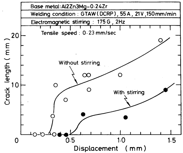
Fig. 9 Relation between crack length and displacement at a constant tensile speed of 0.23 mm/sec for 0.24%Zr containing alloy with and without electromagnetic stirring
