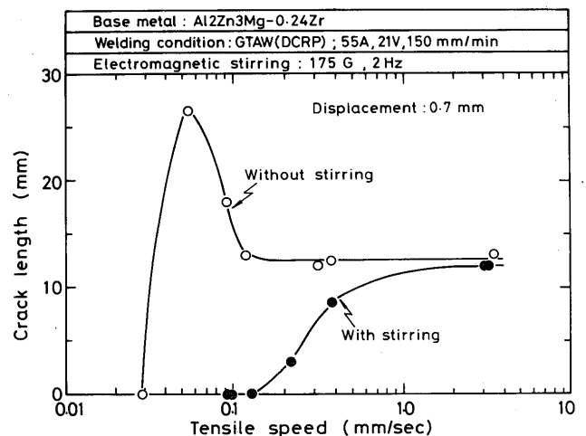
Fig. 7 Relation between crack length and tensile speed under a constant displacement of 0.7 mm for 0.24%Zr containing Al-2%Zn-3%Mg alloy with and without electromagnetic stirring.
