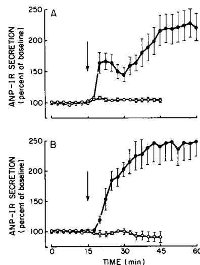
Figure 3. Effect of isoproterenol and phenylephrine on ANP-IR secretion by paced rat left atria. (A) Rat left atria paced at 3 Hz were continuously superfused with 0.1 \mu\text{M} isoproterenol in the absence ( \bullet , n = 6 atria) or presence ( \circ , n = 6 atria) of 1 \mu\text{M} propranolol beginning at 15 min (arrow). Basal ANP-IR secretion was 198 ± 25 pg/ml. (B) Rat left atria paced at 2 Hz were continuously superfused with 10 \mu\text{M} phenylephrine and 1 \mu\text{M} propranolol in the absence ( \bullet , n = 6 atria) or presence ( \circ , n = 3 atria) of 10 \mu\text{M} phentolamine beginning at 15 min. Basal ANP-IR secretion was 158 ± 24 pg/ml.
