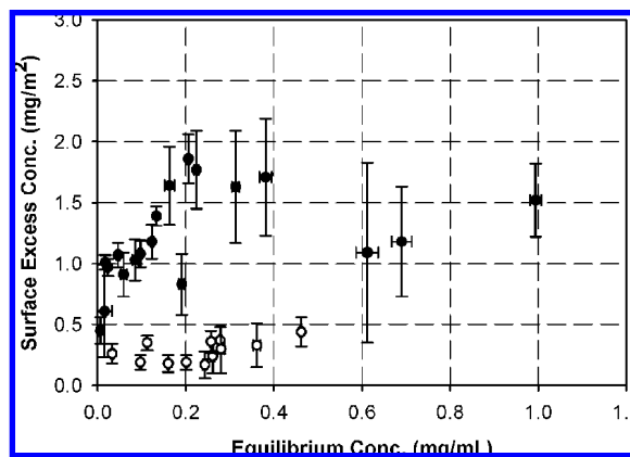
FIGURE 2. Adsorption isotherms of PMAA 15 -PSS 811 (○ open circles) and PMAA 15 -PBMA 43 -PSS 811 (● closed circles). The samples were in 1 mM NaHCO 3 solution.
