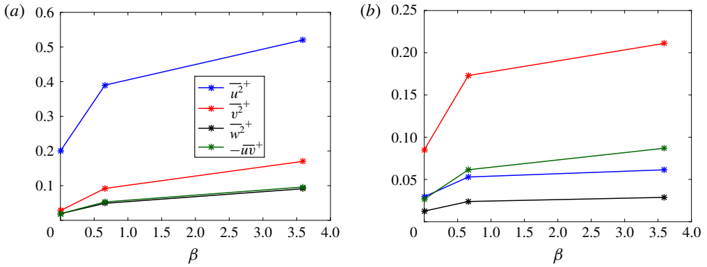
FIGURE 12. (a) Integral of the inner-scaled pre-multiplied spanwise power-spectral density of the various Reynolds stresses (see figure 11) with respect to \lambda_z^+ for values of \lambda_z^+ < 44 . (b) Ratio of the integral for values up to \lambda_z^+ < 44 and the integral along the full range of \lambda_z^+ . Analysis for y_n^+ = 15 .
