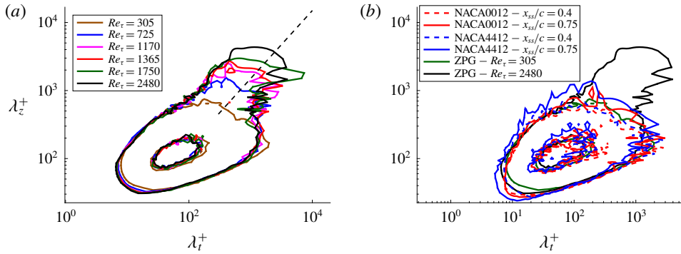
FIGURE 16. Inner-scaled two-dimensional pre-multiplied power-spectral density of the tangential velocity fluctuations k_z k_t \phi_{u_i u_i}^+ at y_n^+ \simeq 15 . (a) ZPG TBL data at different Re_\tau (Eitel-Amor et al. 2014), (b) comparison of the ZPG TBL at different Re_\tau with spectra of the wing sections at x_{ss}/c = 0.4 and 0.75 . The contours correspond to k_z k_t \phi_{u_i u_i}^+ = (0.15, 1) . The dashed straight line in (a) is given by \lambda_z^+ = 1.5\lambda_t^+ .
