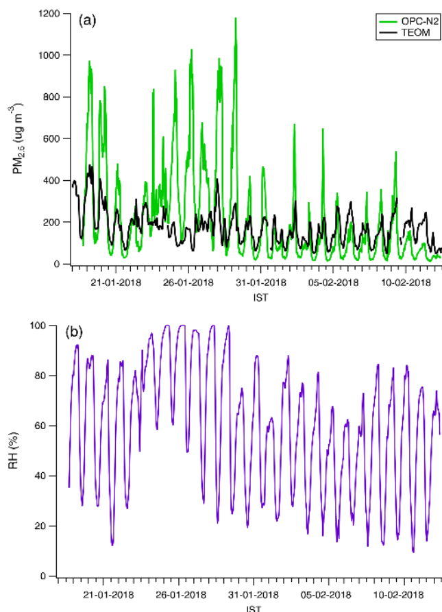
Figure 6. Time series of reported OPC-N2 and TEOM-FDMS PM_{2.5} mass concentrations (a) and ambient RH (b) at IIT Delhi.
