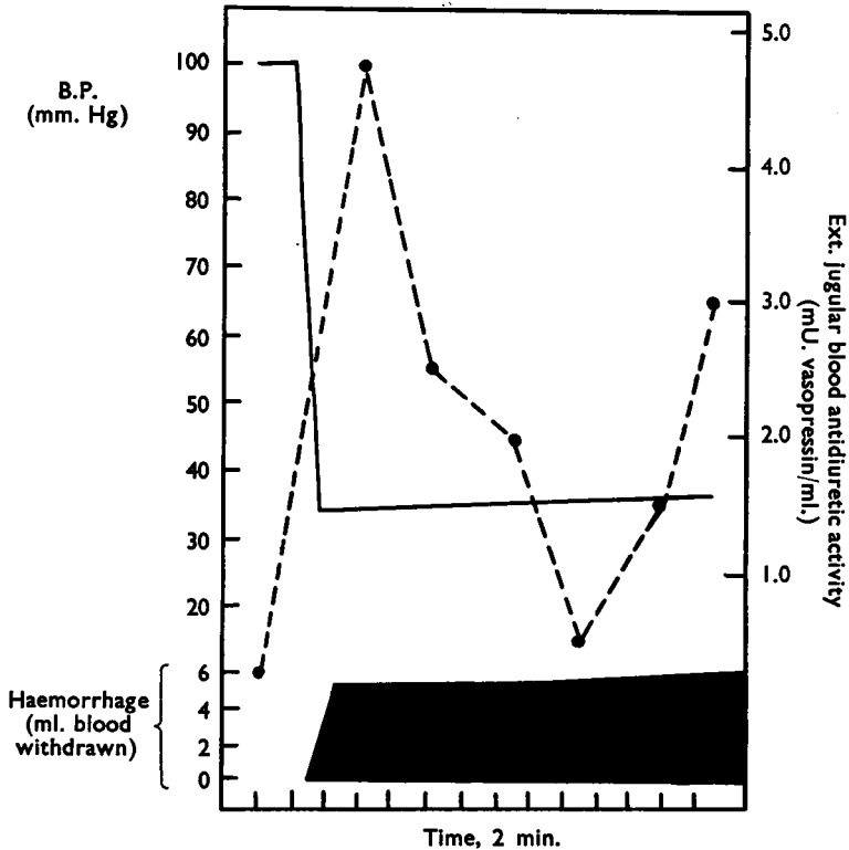
FIG. 4.—Effect of rapid haemorrhage on blood pressure, and antidiuretic activity in external jugular blood. 5.5 ml. blood was maintained at 33–37 mm. Hg. — blood pressure, mm. Hg; • — • mU. vasopressin/ml. blood.
