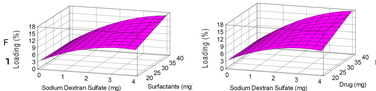
Fig 1: Effect of different factors on drug loading of dextran sulfate-containing SLNs
