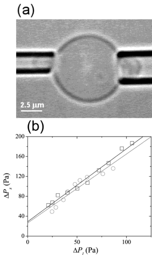
Figure 3. Dual-pipet measurement of the bending rigidity k_c (e.g., OB18 ). (a) A vesicle is partially aspirated into two pipets with different radii ( R_{pl} and R_{ps} ). The larger pipet suction \Delta P_l is used to take up excess area, while the smaller pipet aspiration pressure \Delta P_s deforms a small region of the membrane. (b) Corresponding aspiration curves for two different vesicles. The thermodynamic analysis of Zhelev et al. (ref 31), leading to eq 3, is used to extract k_c .
