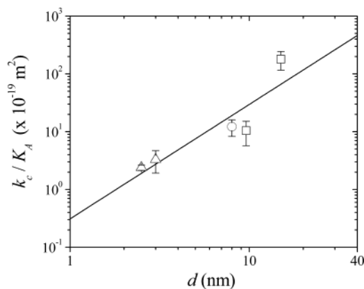
Figure 4. Scaling of k_c with membrane hydrophobic thickness d . Data are shown for DMPC (triangle) (ref 26), SOPC (triangle), OE7 (circle) (ref 9), OB2 (square), and OB18 (square) vesicles. OB18 data are obtained by dual-pipet measurements, whereas all other data come from single-pipet measurements. The line is a least-squares fit, giving a scaling exponent of 2.0 ( R^2 = 0.809 ) as predicted by eq 1.
