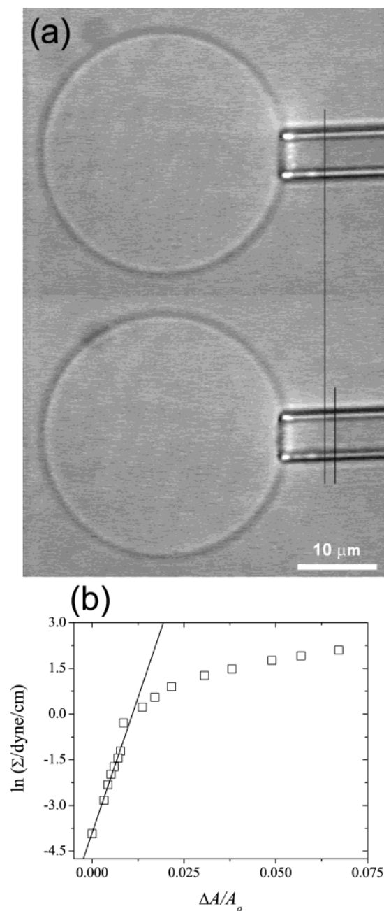
Figure 2. Single-pipet measurements of the bending rigidity k_c (e.g., OB2 ). (a) Micropipet aspiration suppresses the membrane fluctuations at low tensions, smoothing out excess area in the membrane and resulting in an increased projection length \Delta L (ref 30). (b) Corresponding plot of imposed tension vs area dilation to determine k_c . The slope is 8\pi k_c/k_B T from eq 2.
